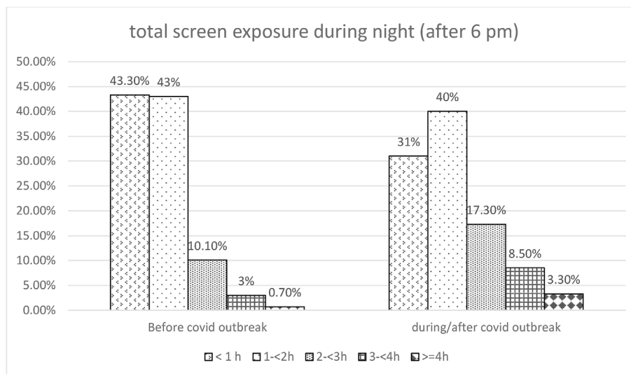
Fig. 3. Chart showing a reduction of children using devices for less than 2 h in the evening time (after 6 p.m.) with a concomitant increase of those exposed for longer time.
